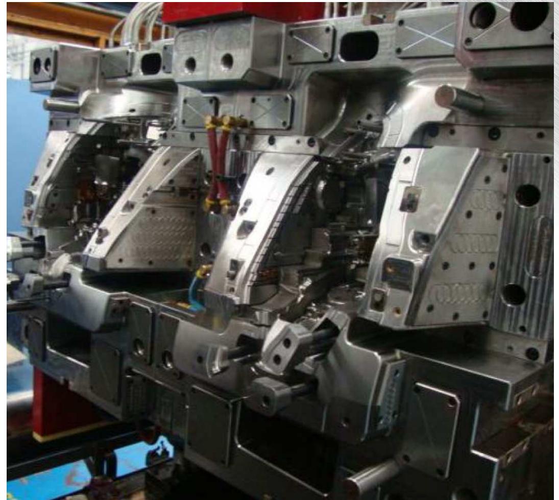
Daimler Headlamp Housing
